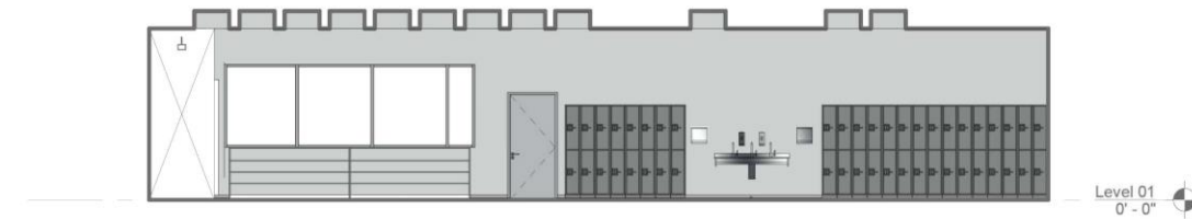
1 | INTERIOR ELEVATION - WELDING SHOP NORTH A1.21 1/8" = 1'-0"
